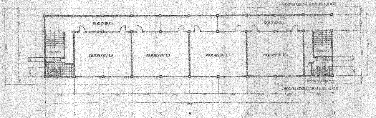
R3 BUILDING TYPICAL 2ND TO 3RD FLOOR PLAN SCALE: 1/200 S.F.T.S.
